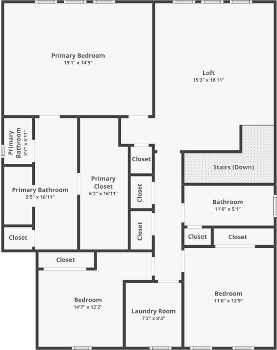
FLOOR 2
